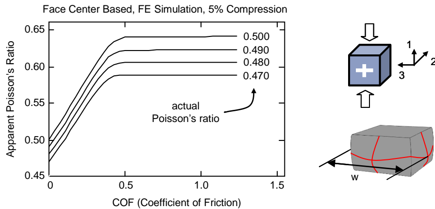
Figure 6: Finite element study of the dependence of the apparent Poisson's ratios on coefficients of friction when compressing an isotropic elastic cube (1x1 dimensions).
